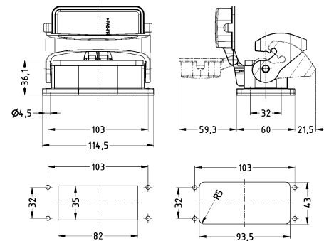
Panel cut out Front mounting / Rear mounting
