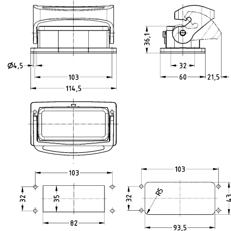
Panel cut out Front mounting / Rear mounting
