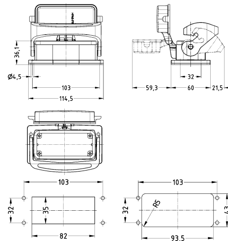
Panel cut out Front mounting / Rear mounting
